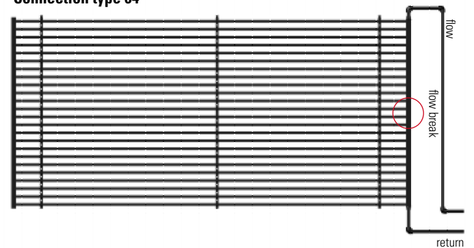
Connection type 64
