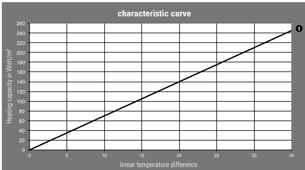
characteristic curve
